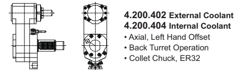
4.200.864 External Coolant 4.200.950 Internal Coolant • Radial, Left Hand • Collet Chuck, ER32 • PRECI-FLEX®
