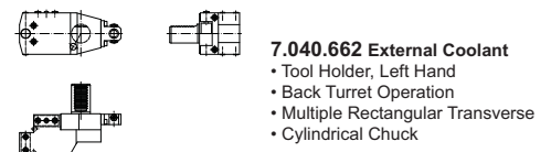
7.070.085 External Coolant • Tool Holder, Radial • Left Hand Rectangular Transverse
